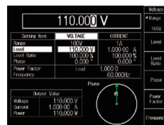
Example of voltage setting screen
